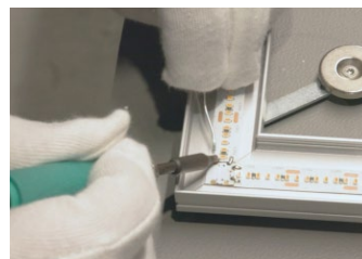
Merging LED flex stripes and aluminum profiles
